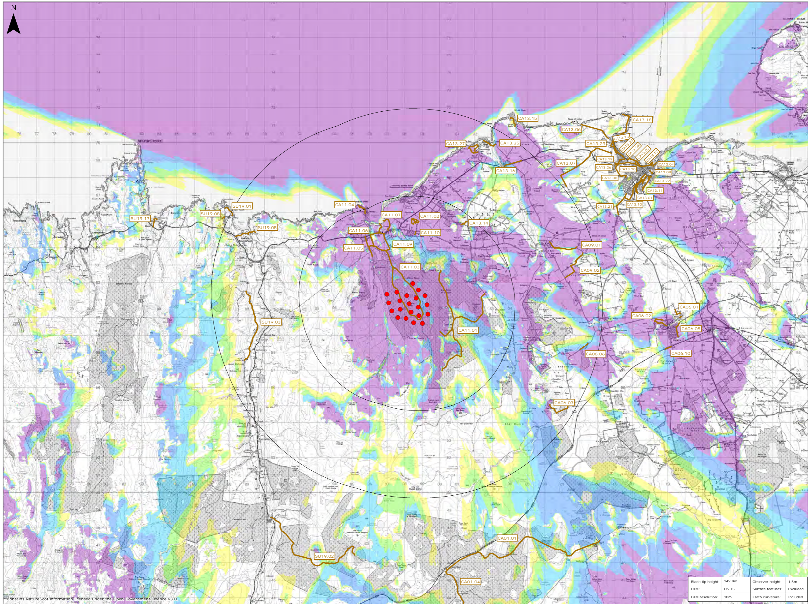
Figure 9.16: Core Paths with Blade Tip ZTV
